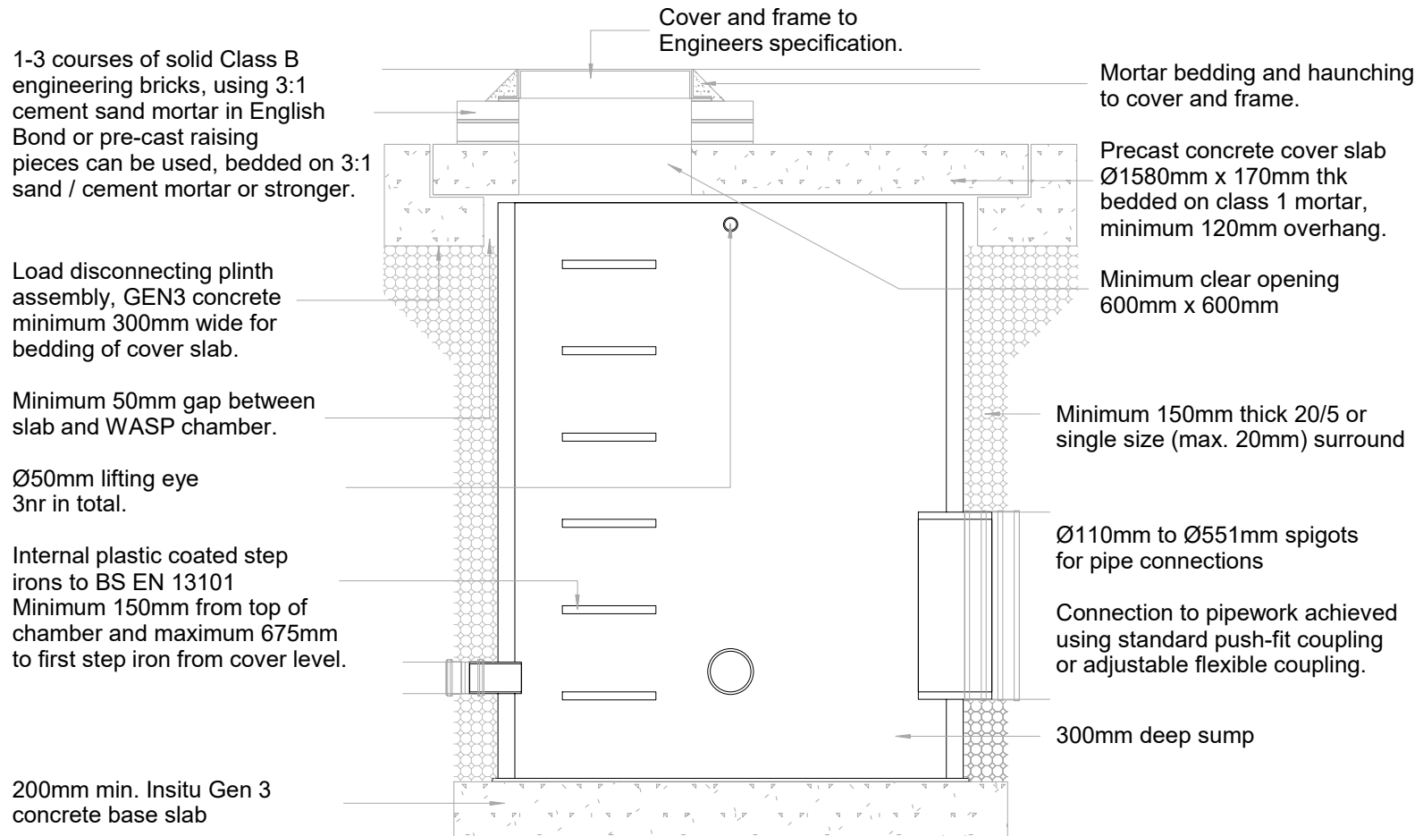
INSTALLATION DETAIL WASP05350 Series Prefabricated Catchpit Chamber Ø1500 up to 2.5m deep chamber By SEL Environmental Tel: 01254 589987
